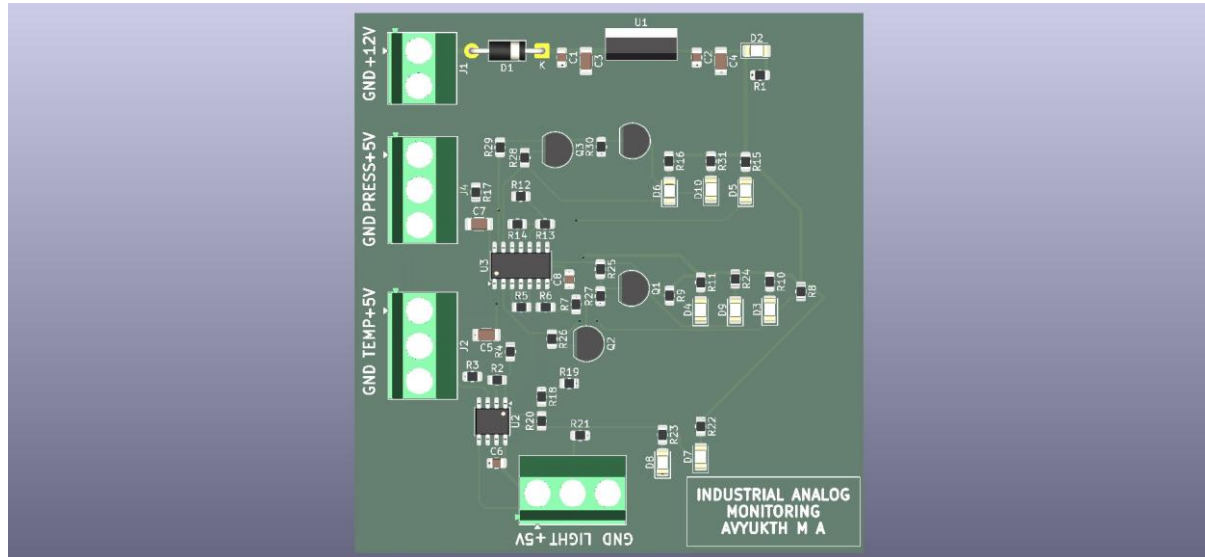
Figure 1 — Industrial Condition Monitoring Board (KiCad 3D Render, Top View)
